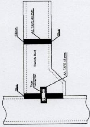
Branch Duct Connection
